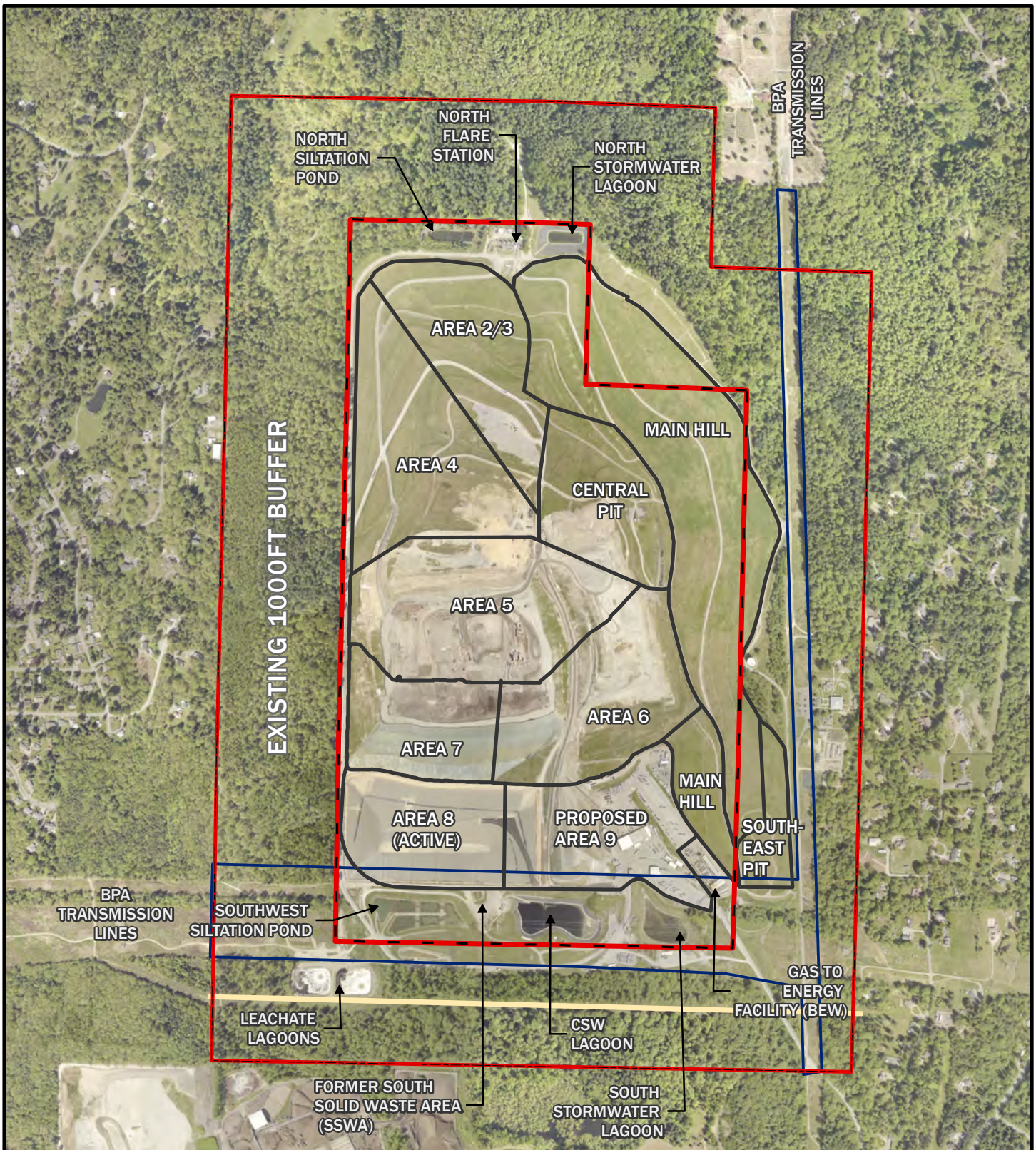
Figure 1-3. Landfill Disposal Areas in the Cedar Hills Regional Landfill.
