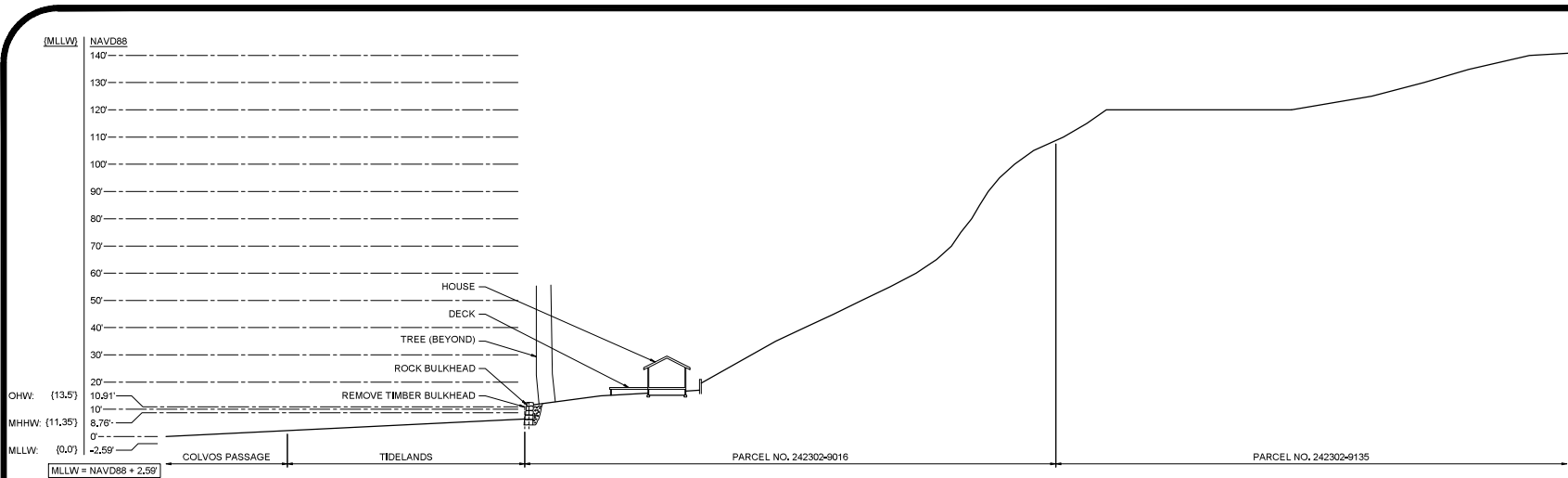
SECTION - PROPOSED BULKHEAD 1" = 20'-0"
