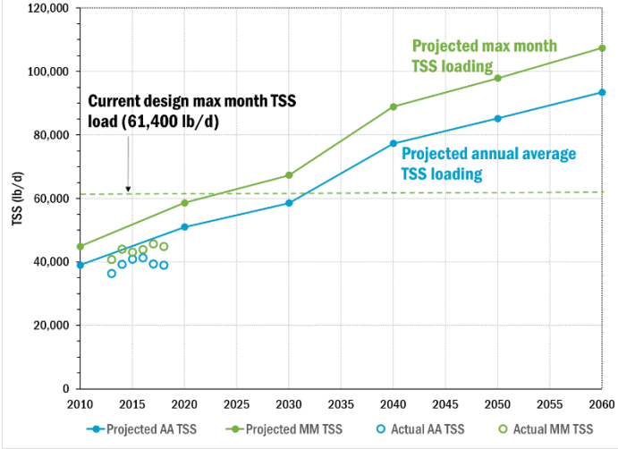
FIGURE 15 Historical and Projected TSS Loadings to Brightwater
