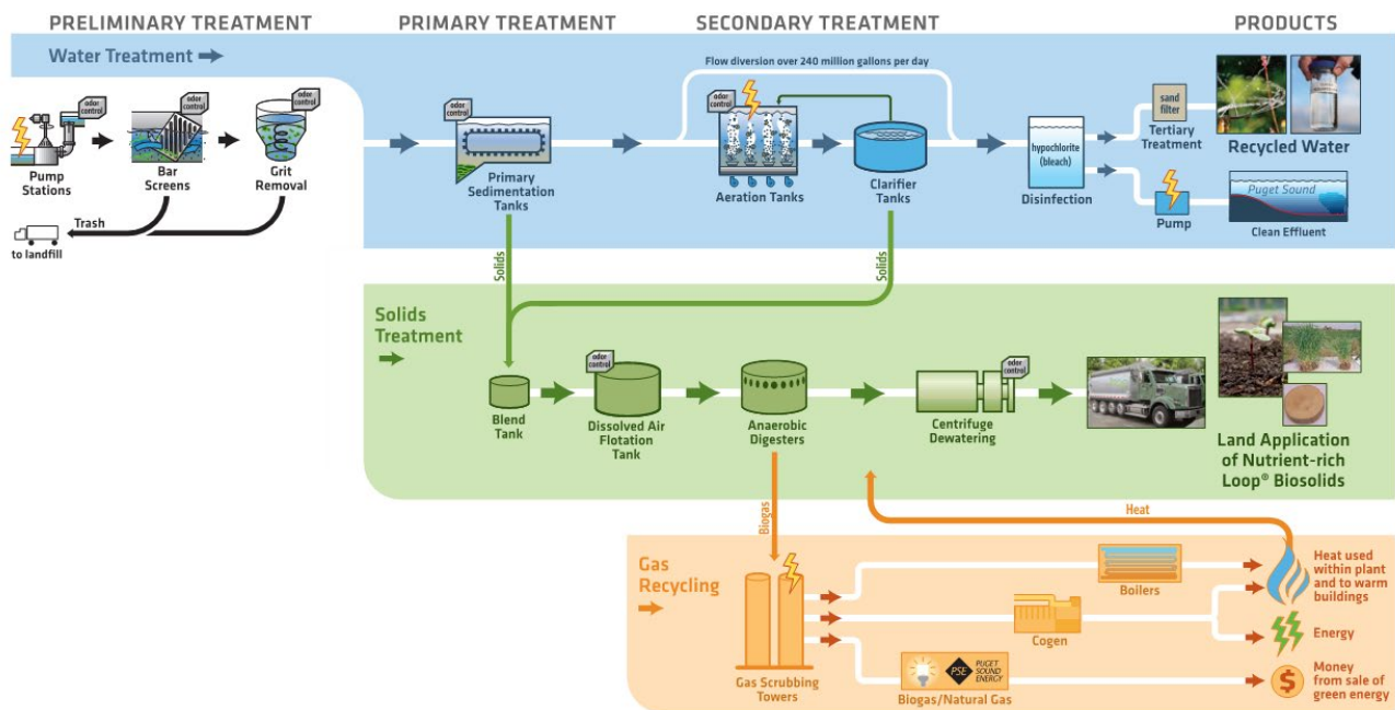
FIGURE 2. South Plant Process Flow Schematic
