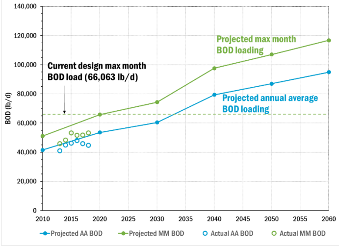
FIGURE 14 Historical and Projected BOD Loadings to Brightwater
