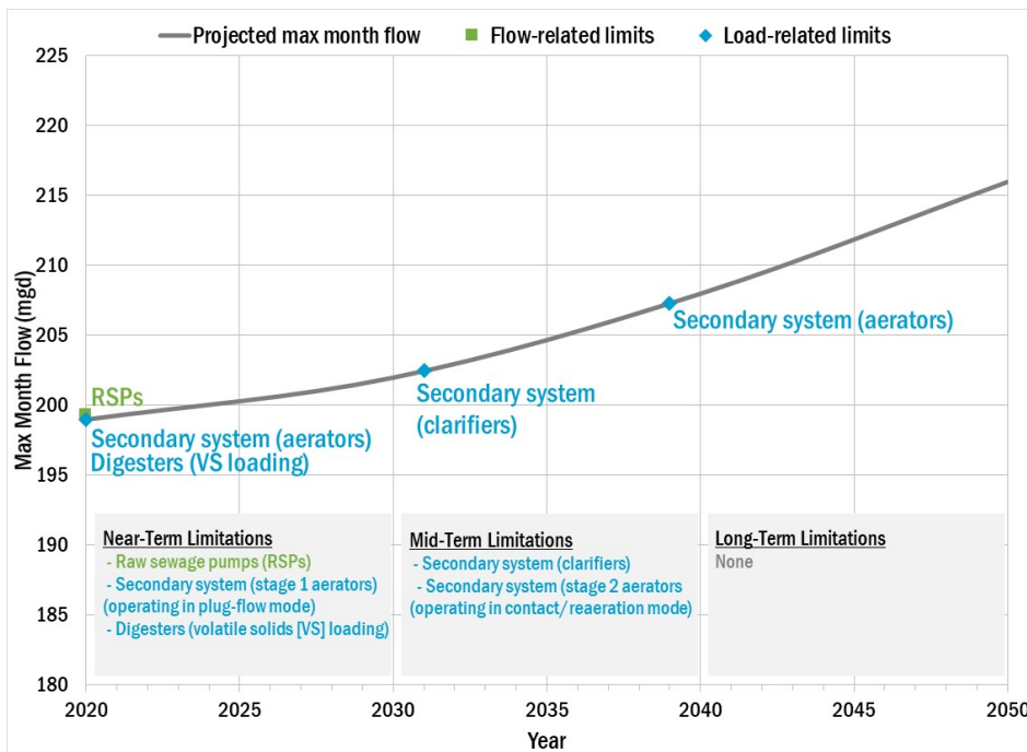
FIGURE 11 West Point Timeline of Unit Process Capacity Constraints
