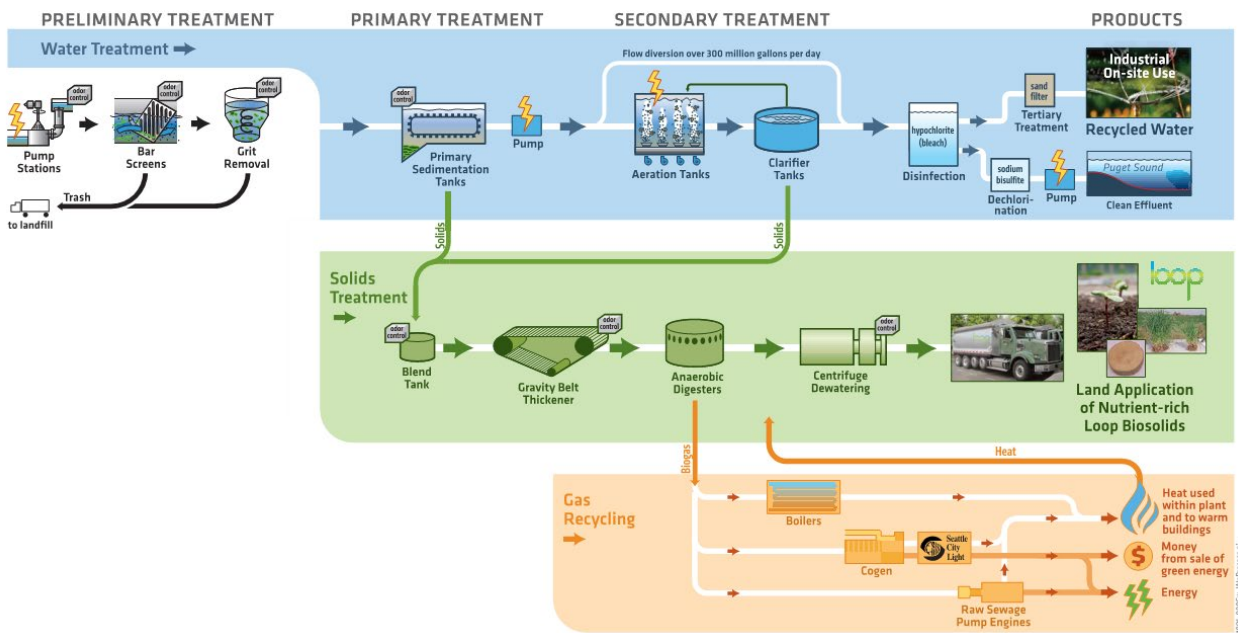
FIGURE 7 West Point Process Flow Schematic
