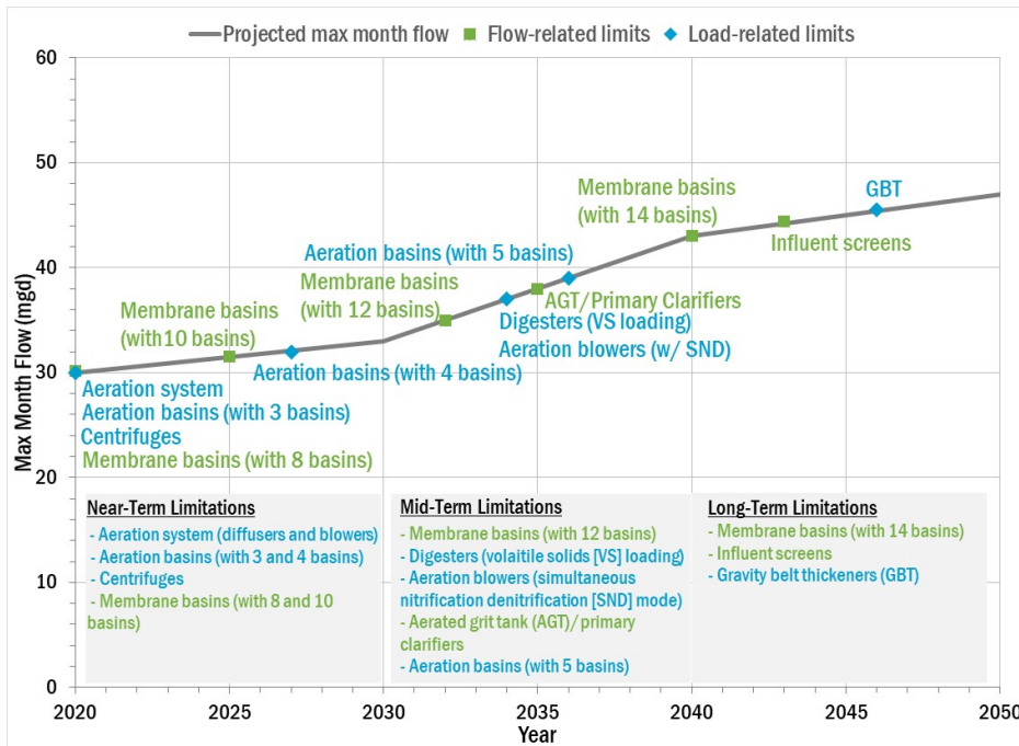
FIGURE 16 Brightwater Timeline of Unit Process Capacity Constraints
