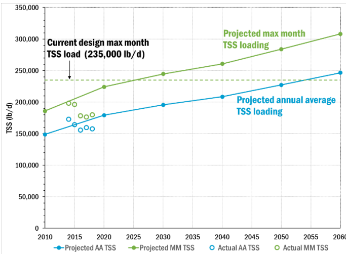
FIGURE 5 Historical and Projected TSS Loadings to South Plant
