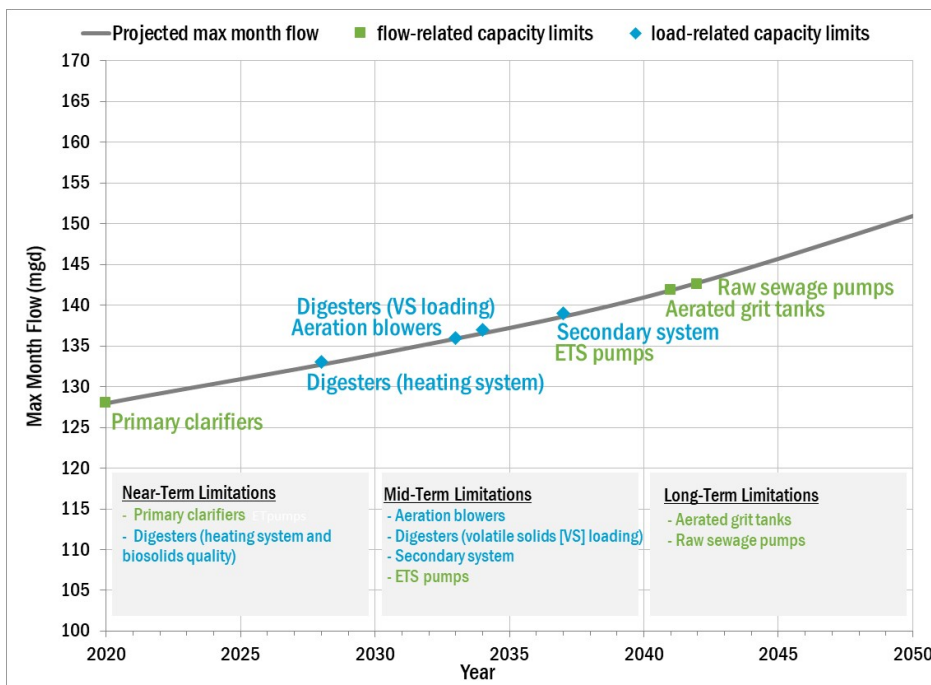
FIGURE 6 South Plant Timeline of Process Capacity Constraints
