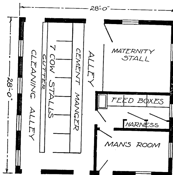
Design 1748—For 7 Cows
