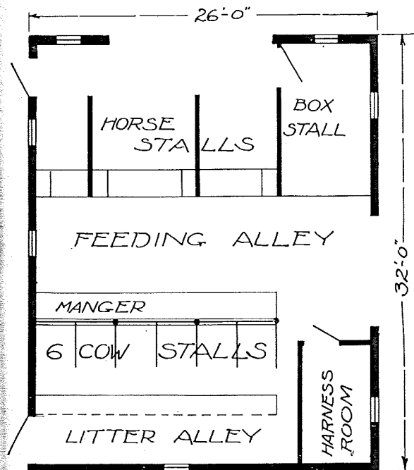
Design 1808—For 6 Cows and 4 Horses
