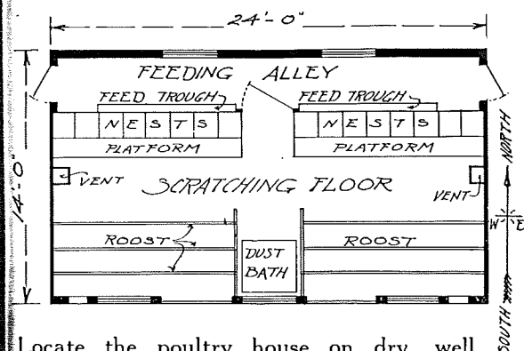
Design 3034—Chicken House
