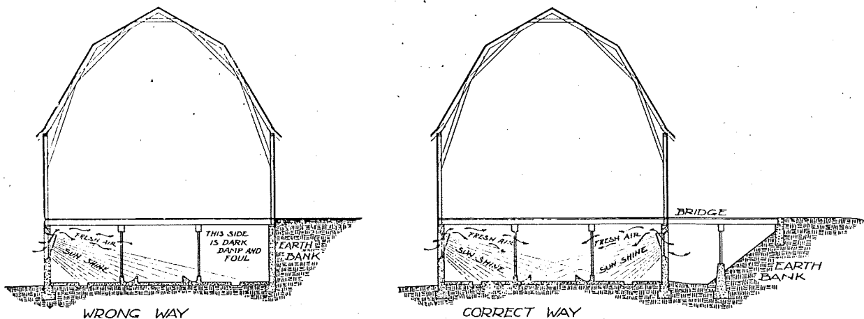
Two Methods of Building a Bank Barn
