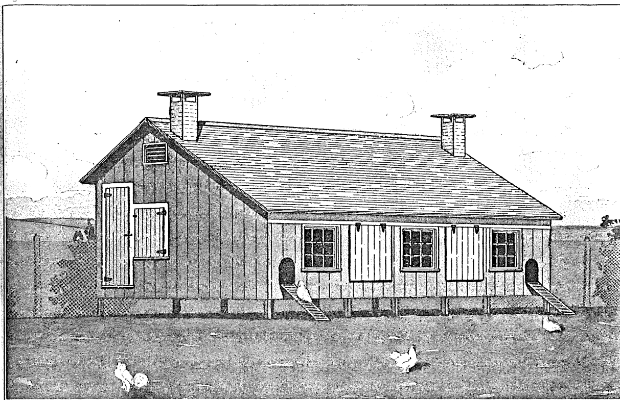
Design 3034—Chicken House
