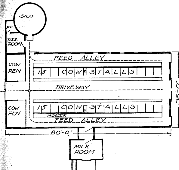
Design 2419—For 30 Cows
