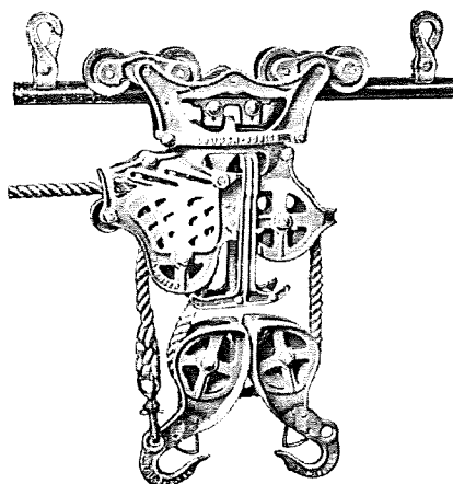
Louden Junior Sling Carrier.
