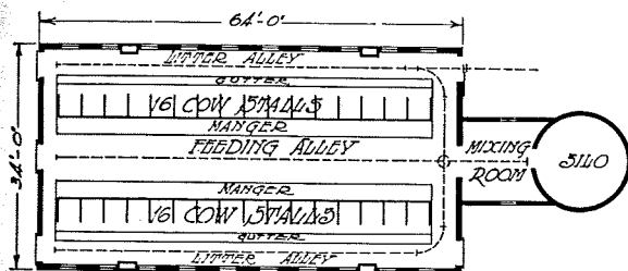
Design 3982—For 32 Cows
