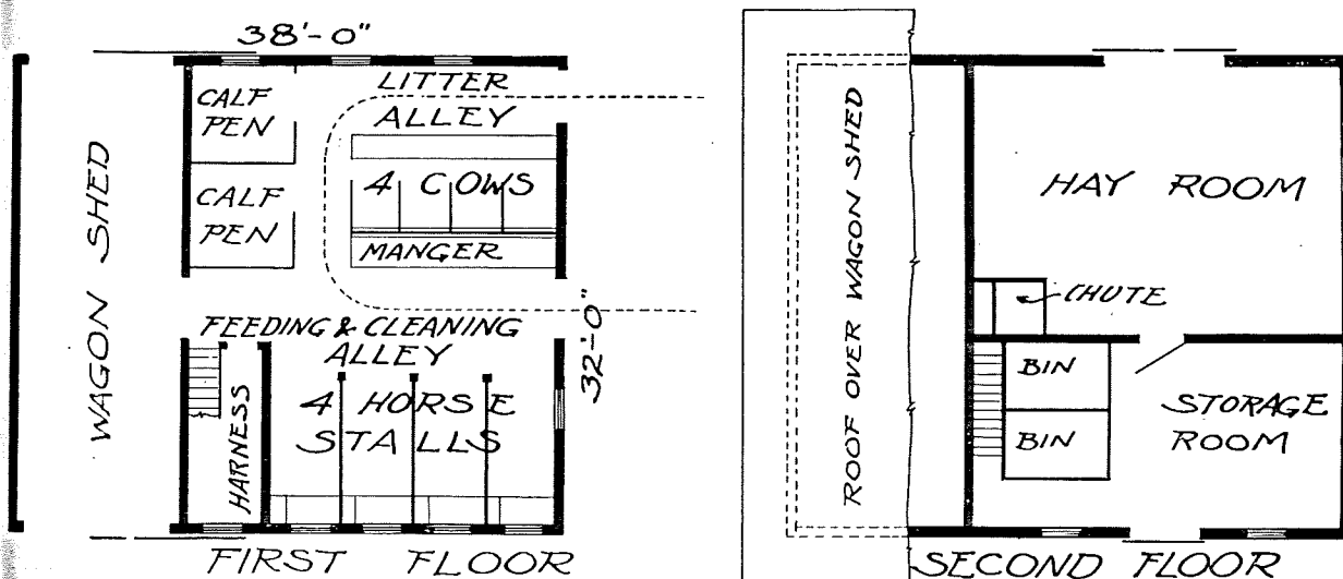
Design 2420 — For 4 Cows and 4 Horses
