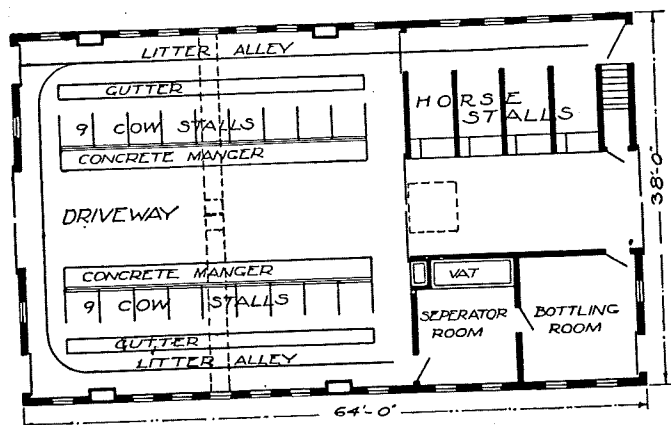
Design 2162—For 18 Cows and 4 Horses
