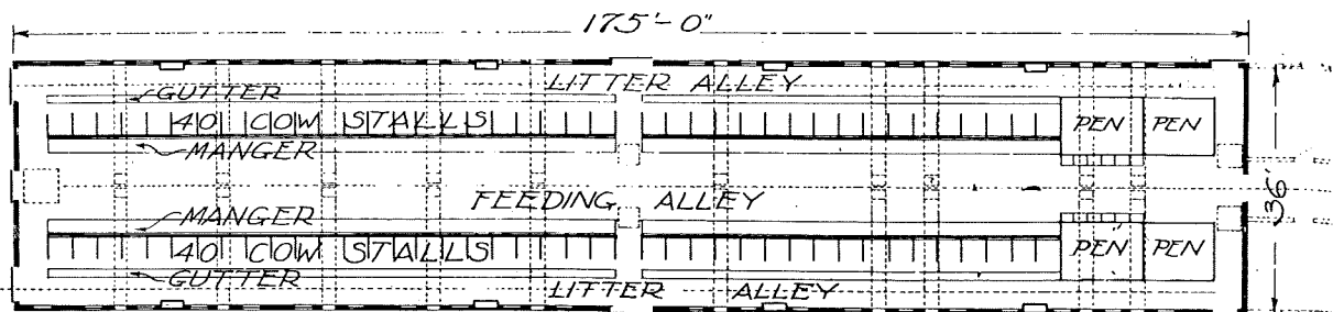
Design 2603 — For 80 Cows
