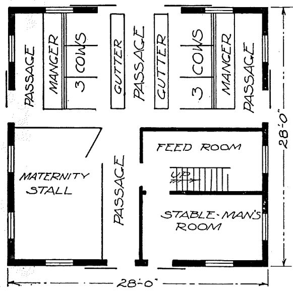
Design 1773—For 7 Cows
