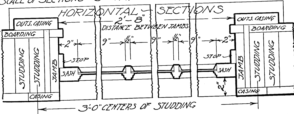
SCALE OF SECTIONS = 3" = 1 FT.
