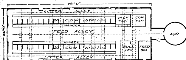
Design 2561—For 40 Cows
