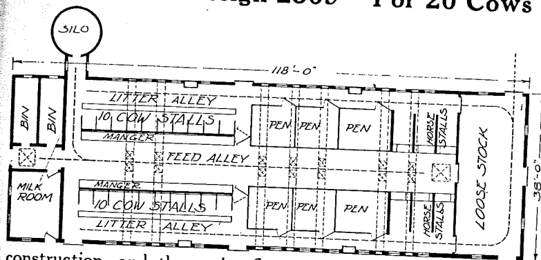
Design 2569—For 20 Cows and 6 Horses
