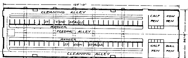
Design 2550 — For 54 Cows
