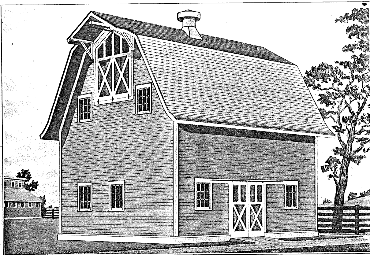
Design 1808—For 6 Cows and 4 Horses
