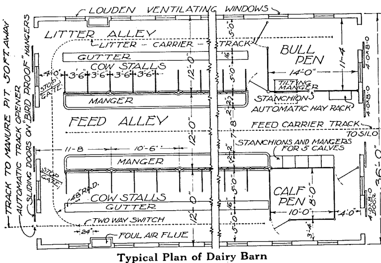
Typical Plan of Dairy Barn
