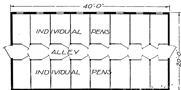
Design 2457B—Hog House with 16 Pens
