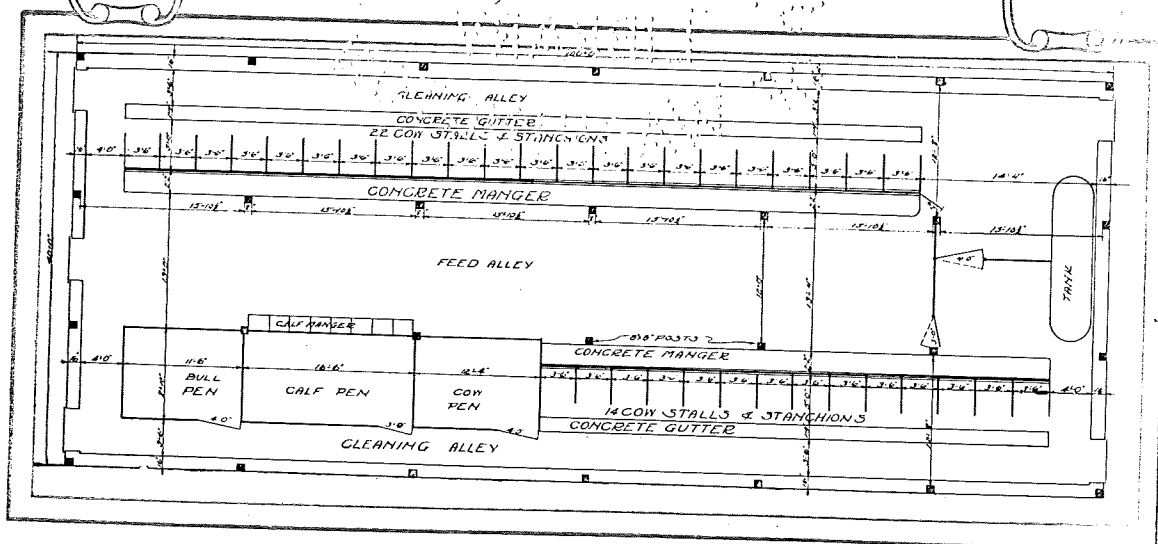
"Tobacco River Ranch"— owned by W. C. Cornwell, Clare, Michigan. This dairy barn was designed by the Loudon Architectural Department and equipped with Cow Stalls, (Fig. 812) Maternity Pens, Calf Pens, and Bull Pen, Emanci- pator Litter Carrier, Double End Feed Carrier, etc., Mr. Cornwell is one of Michigan's progressive dairymen and is giving special attention to breeding pure bred stock.
