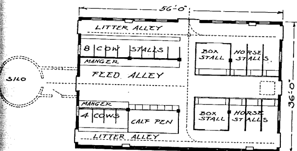
Design 2566A—For 12 Cows and 8 Horses
