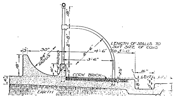
Section of Loudon Cow Stall
