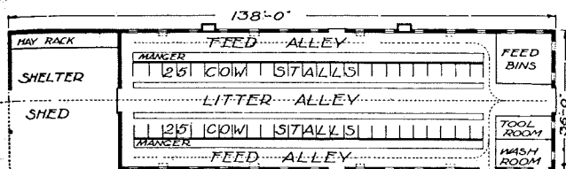
Design 1670—For 50 Cows
