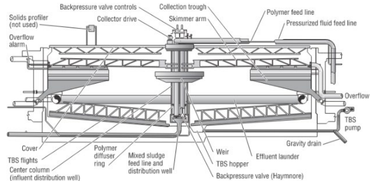
Figure 1-1. DAFT Cross Section (Source: STP Thickening O&M Manual)
