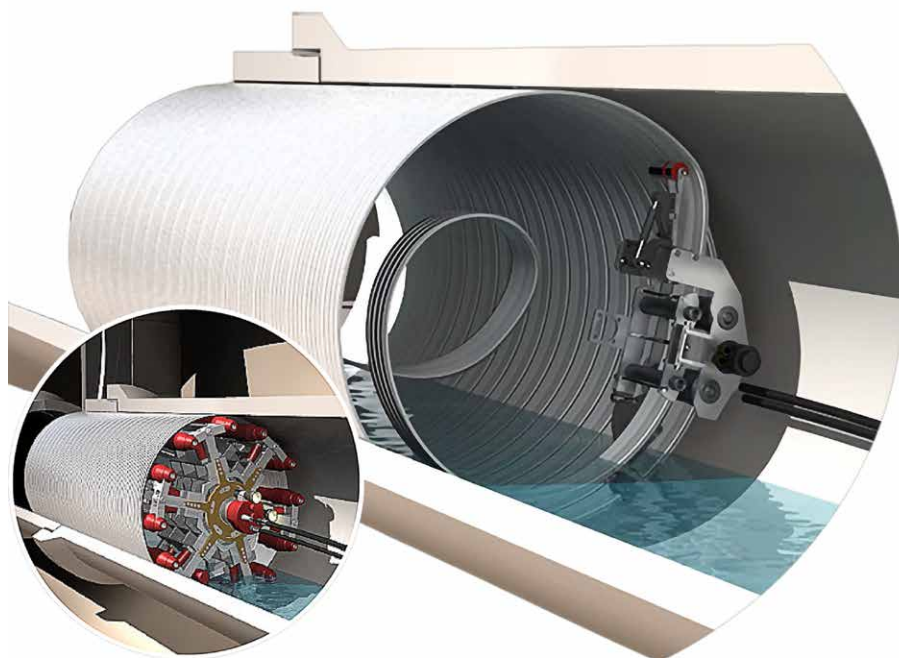
Crews will use spiral wound technology to install the new pipe lining.
