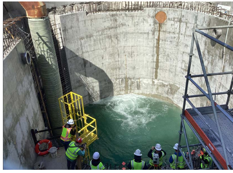
The Ship Canal Water Quality Project is a joint effort between King County and Seattle Public Utilities. The project will capture and store 29 million gallons of polluted water during heavy rains. An underground storage tunnel is being built to hold the stormwater and sewage until there is room to send it to the West Point Treatment Plant. It will control four CSO outfalls for the City of Seattle and two King County outfalls at 3rd Ave. W and 11th Ave. NW. Construction is ongoing.
