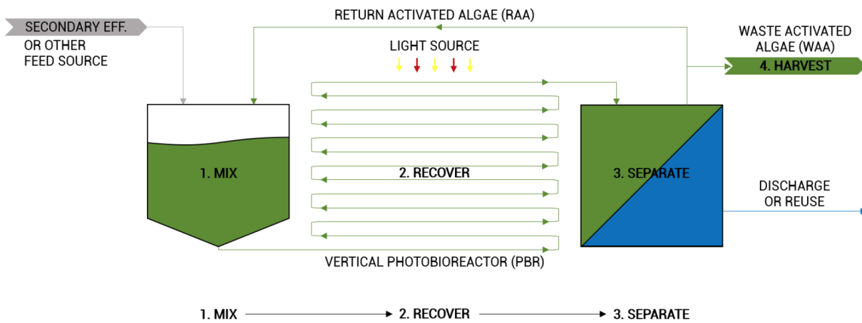
Process flow diagram from CLEARAS Water Recovery
