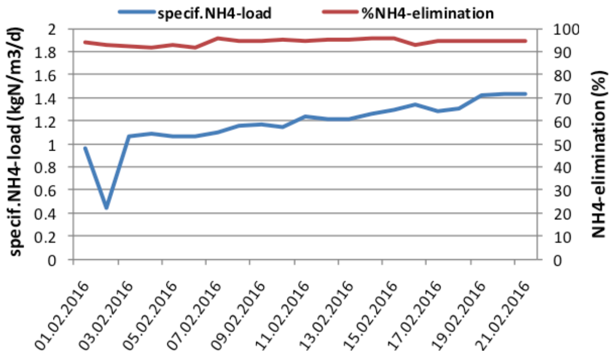
FIGURE 5 – SPECIFIC LOAD AND AMMONIA PERCENT REMOVAL – FEB 2016
