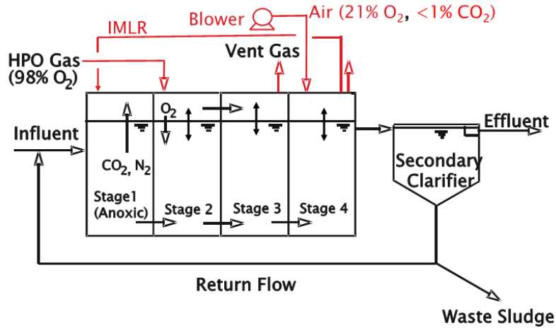
Figure 1. Schematic of HPO process modified for nitrogen removal (MLE-HPO)
