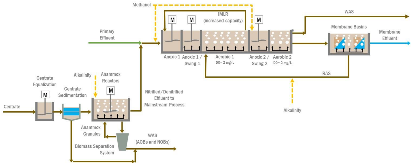
Figure 6. Process flow schematic for Alternative 3B – 4SMB/MBR + sidestream anammox
