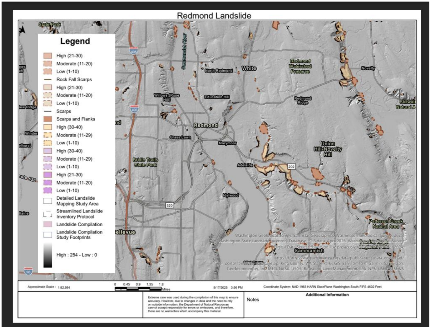
Figure 5: Landslide Hazard Areas
