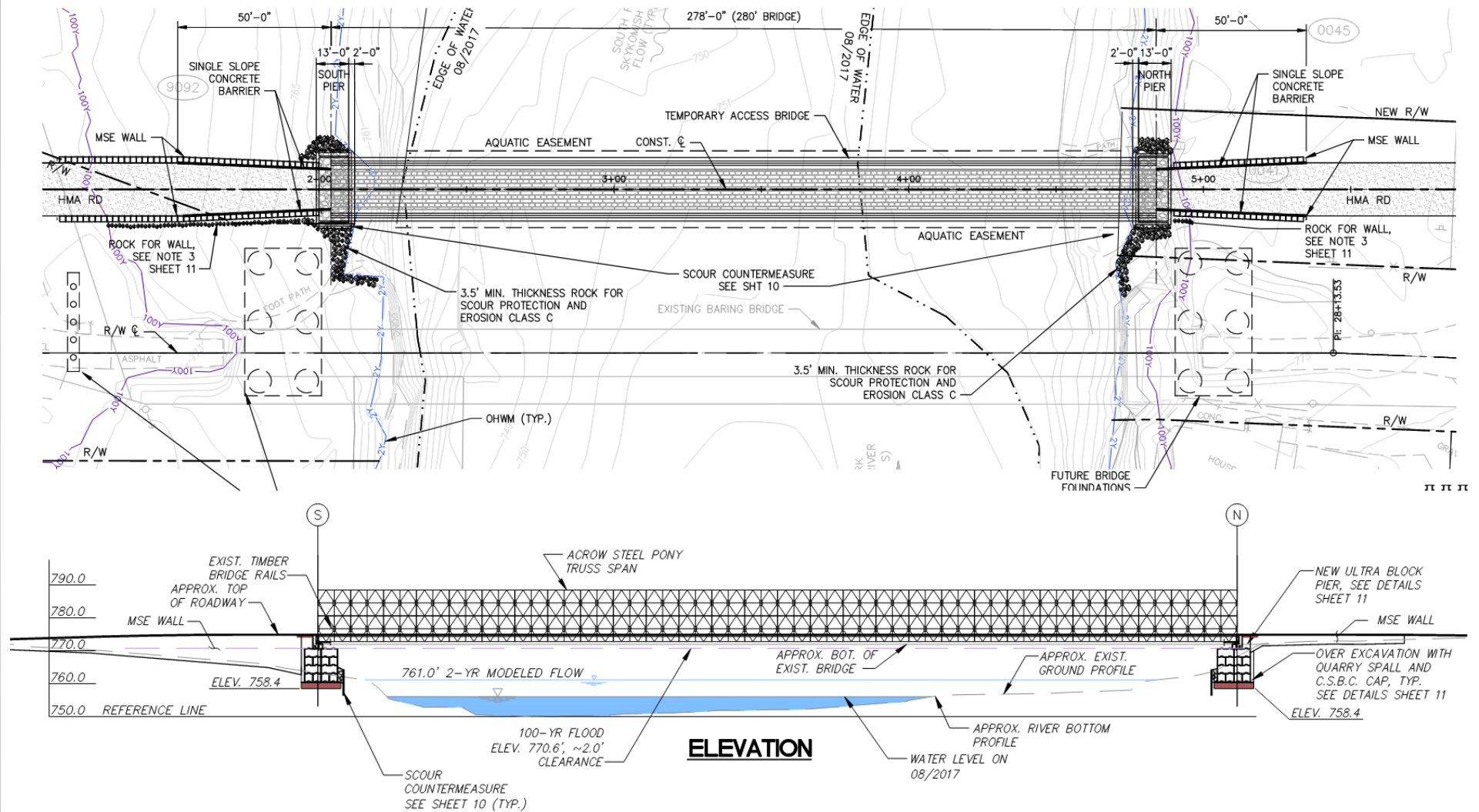
Baring Bridge #509A Replacement
