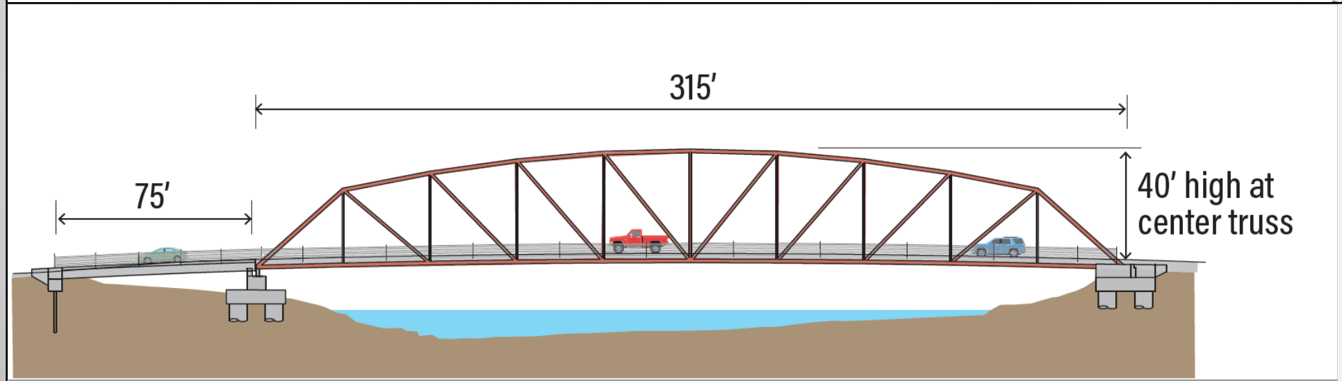
Baring Bridge #509A Replacement
