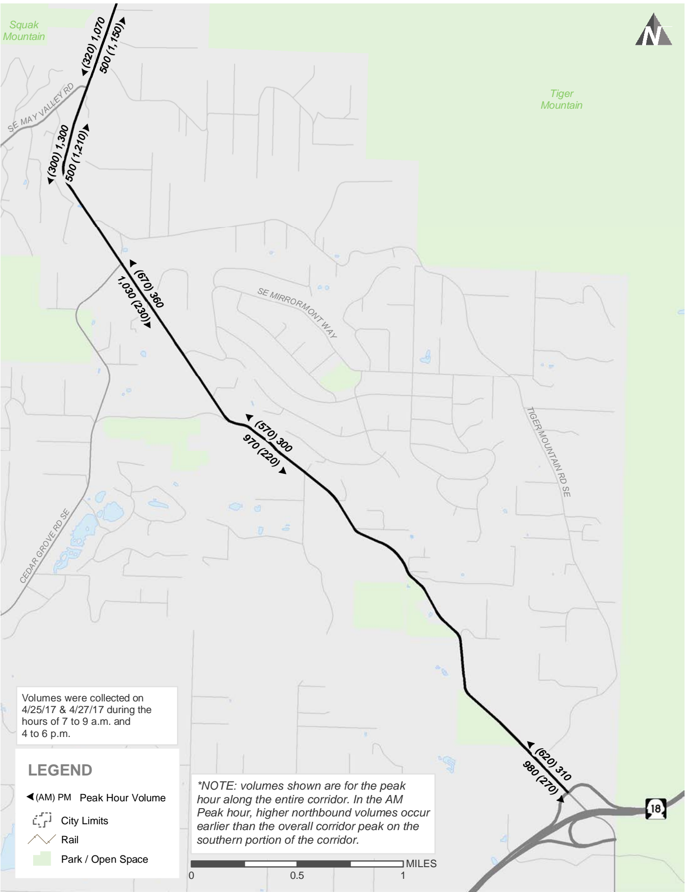
Weekday (2017) AM & PM Peak Hour Roadway Volumes - South
