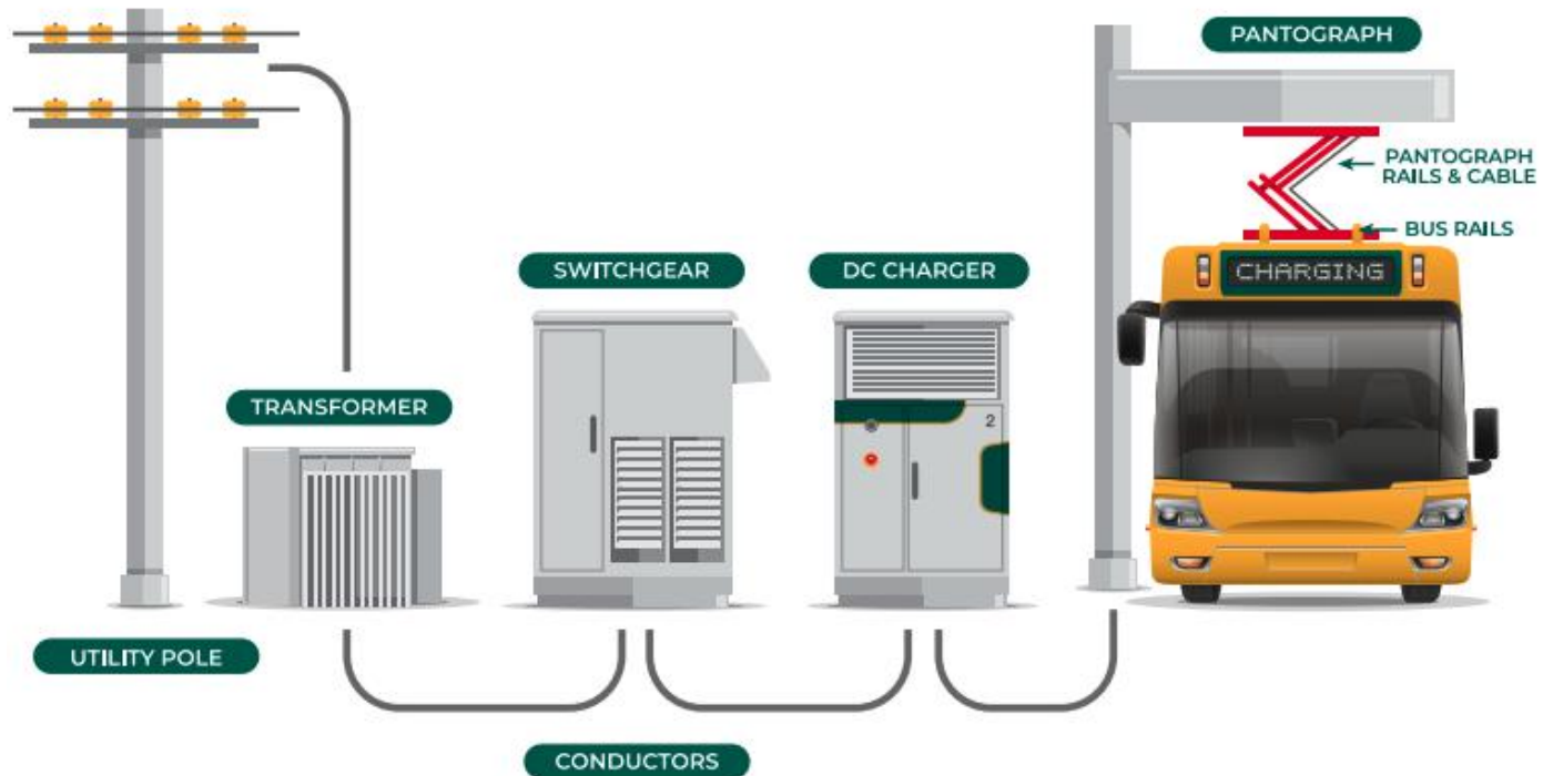
Figure 6. High-level charging infrastructure schematic
