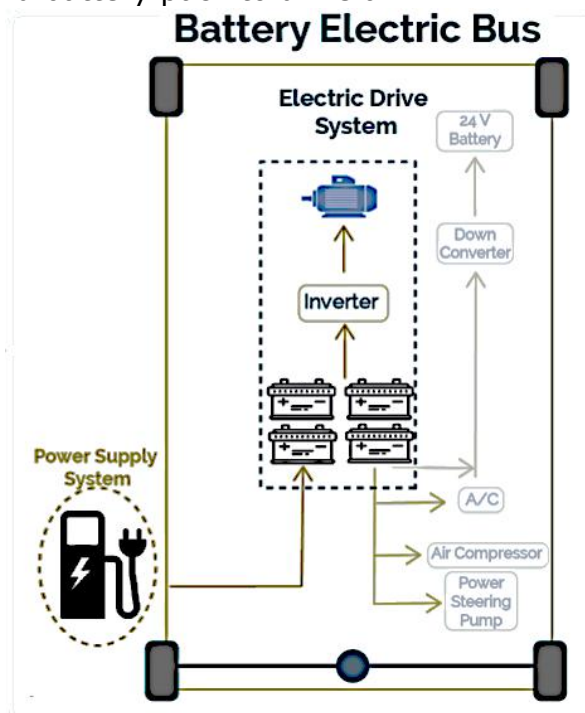
Figure 1. Basic Schematic of a Battery-Electric Bus
