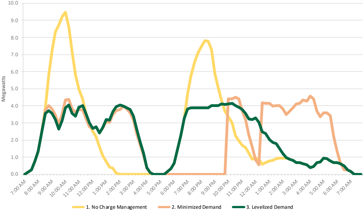
Figure 1. Charging Demand Over One Day, Scenarios 1-3
