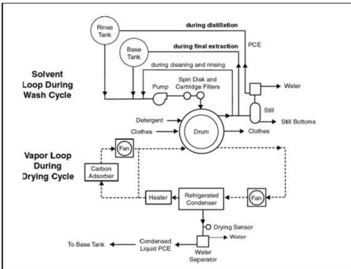
Figure 1. Simplified dry cleaning process diagram
