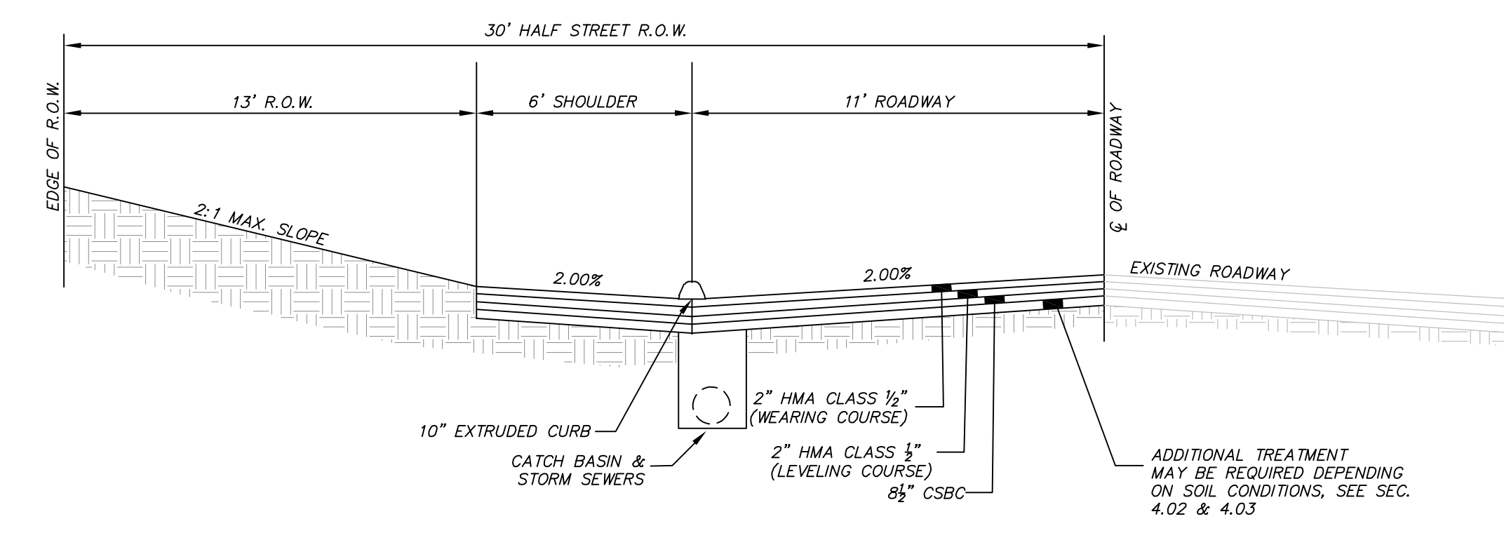
332ND AVE SE, STA 30+32.69 - 31+64.21 (URBAN SUBACCESS ROAD, EXTRUDED CURB TYPE ROADWAY) 2016 RCRDCS NTS
