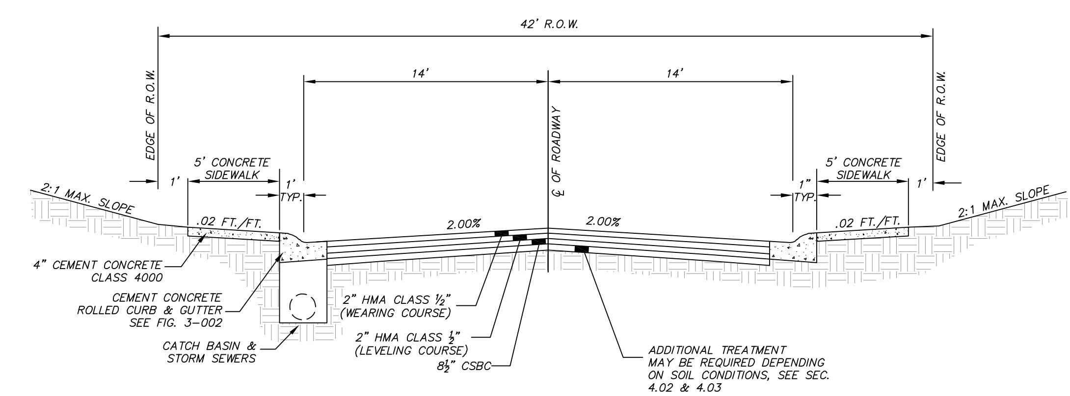
ROAD A, STA 20+00.00 - 21+45.00 (URBAN SUBACCESS ROAD, ROLLED CURB TYPE ROADWAY) 2016 RCRDCS NTS
