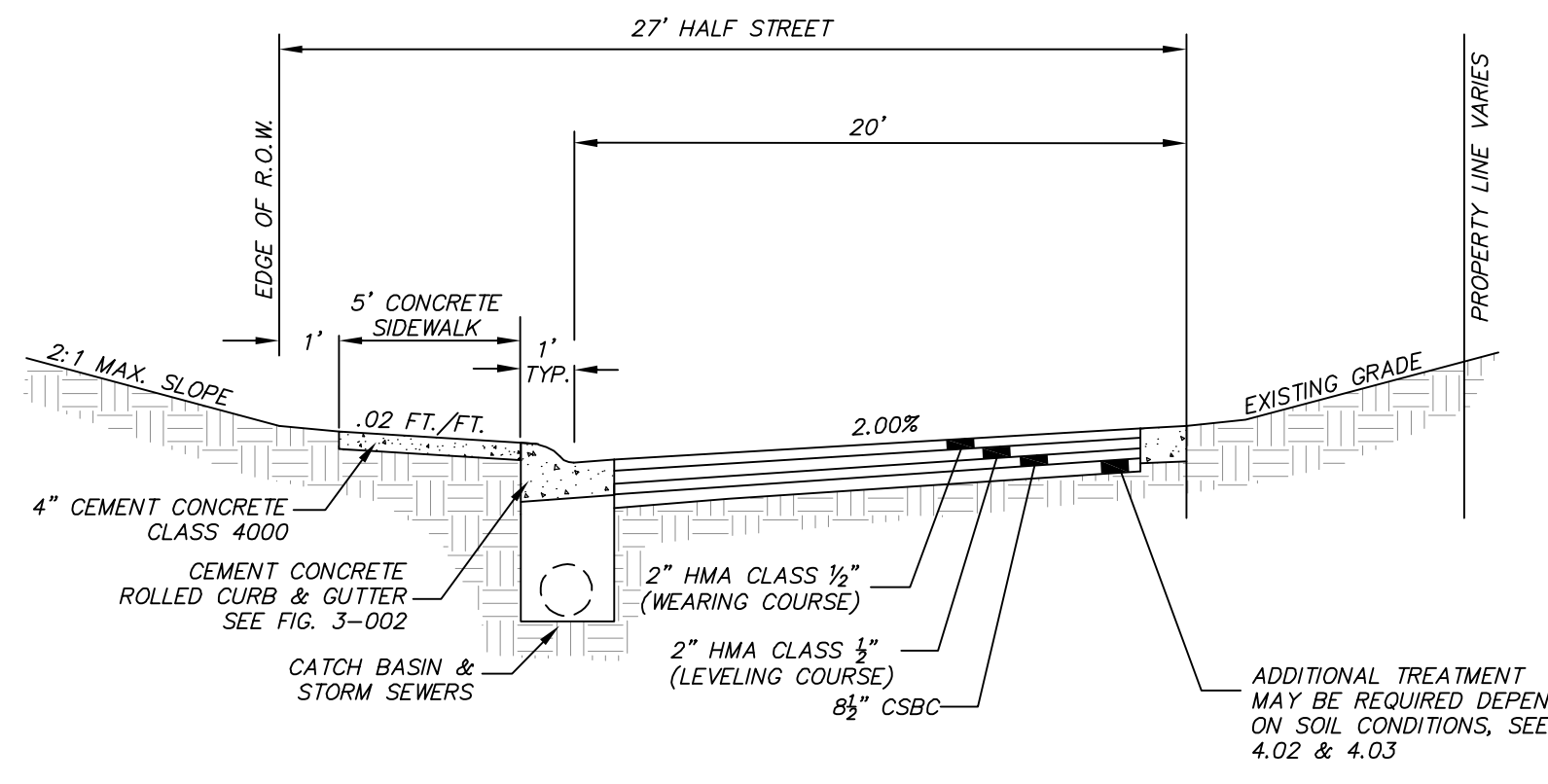
SE 41ST ST, STA 10+37.88 - 18+86.30 (URBAN SUBACCESS ROAD, ROLLED/VERTICAL CURB TYPE ROADWAY) 2016 RCRDCS NTS
